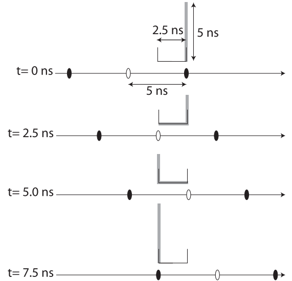
FIG. 6. Schematic time-sequence diagram of circulating and injected bunches, and kicker input pulse for a ring with 100 \text{ MHz} rf system. The grey thick line represents the input pulse, propagating along the electrode. The closed ellipses represent the circulating bunches, and the open ellipse represents the injected bunch. The kicker efficiency is maximized with a length of 0.75 \text{ m} (corresponding to a transit time of 2.5 \text{ ns} , a quarter of the bunch spacing), i.e., the kicker can be fully filled with the input pulse during the transit of the injected bunch without deflecting the circulating bunches.
