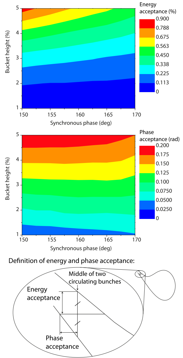
FIG. 10. Energy (top plot) and phase (center plot) acceptance. They are defined as shown schematically at the bottom.
